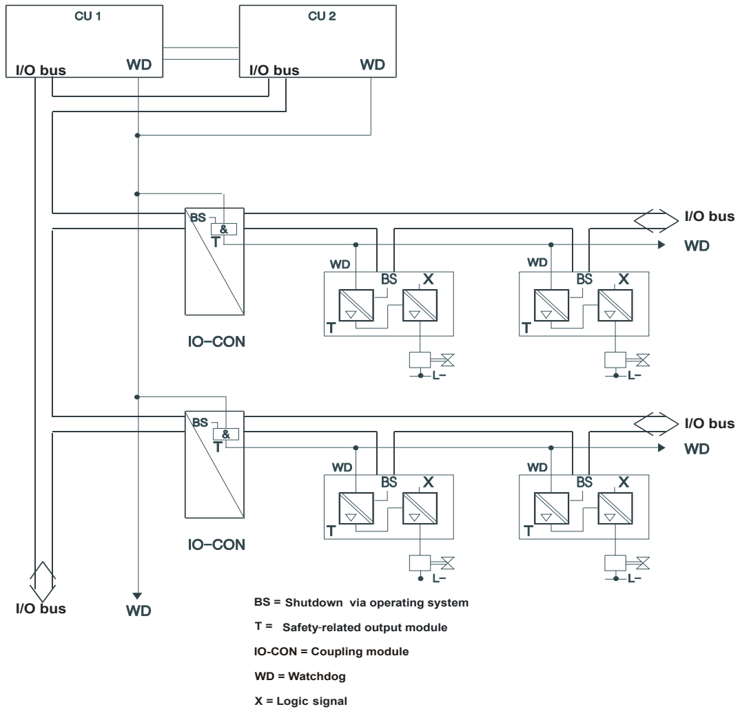
Figure 6: Shutdown ways in the H51q-HS system
