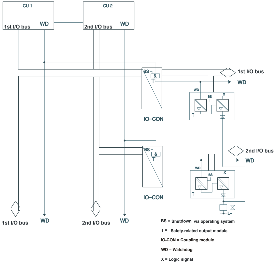
Figure 7: Shutdown ways in the H51q-HRS system
