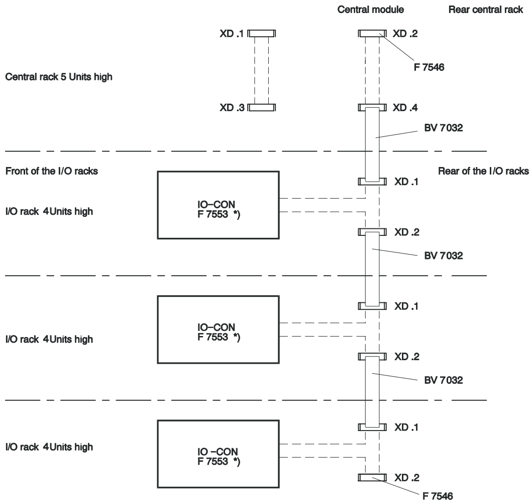
Figure 3: Construction principle of the I/O bus for system H51q-MS
