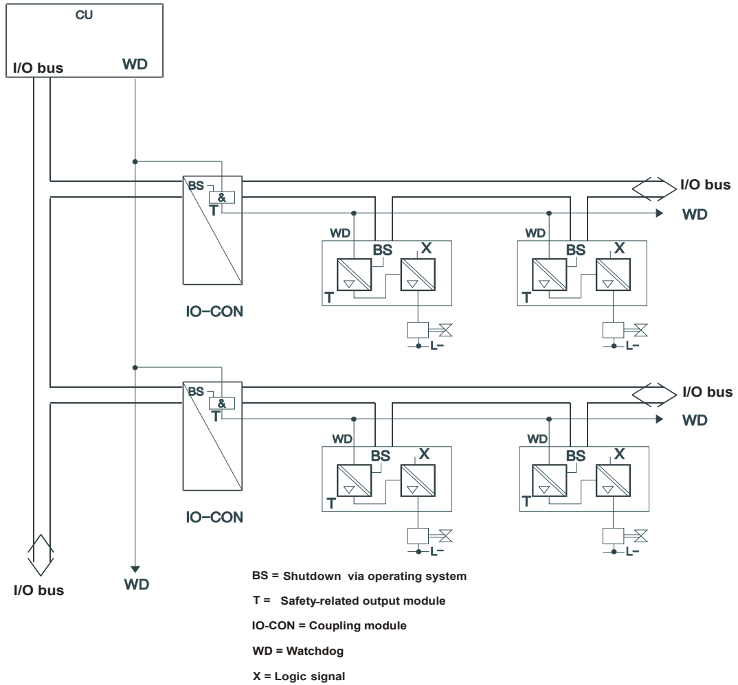
Figure 4: Shutdown ways in the H51q-MS system
