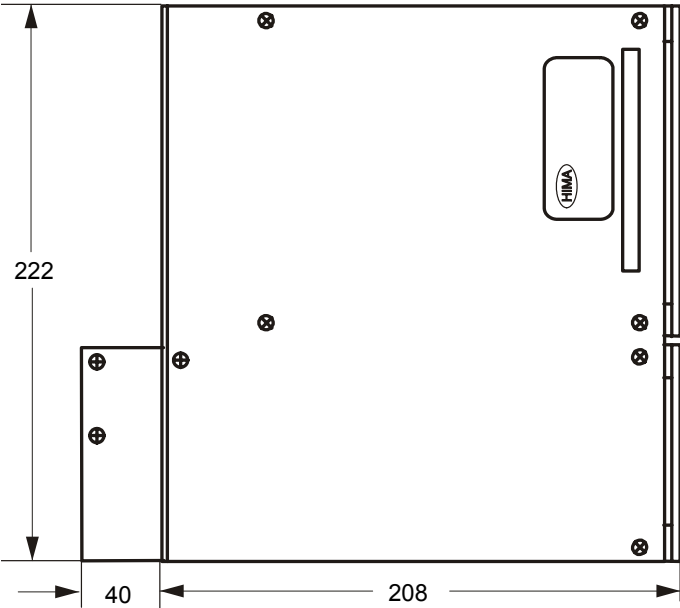
Figure 5: Side view
