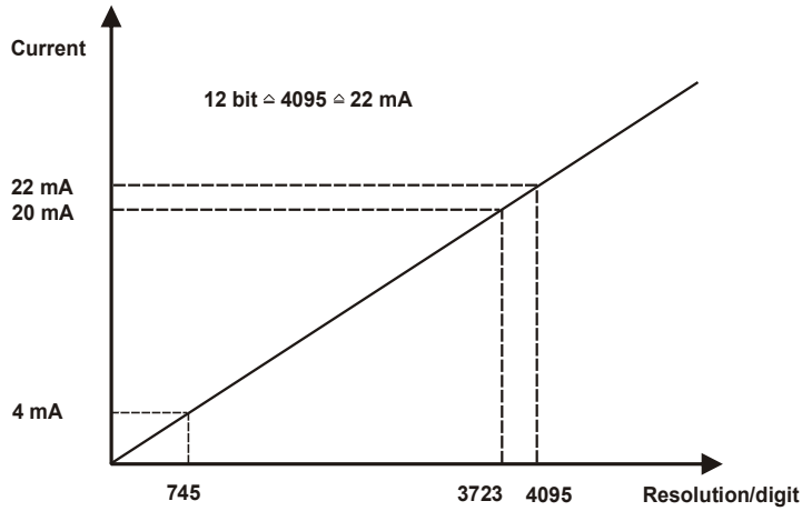
Figure 3: Current inputs
