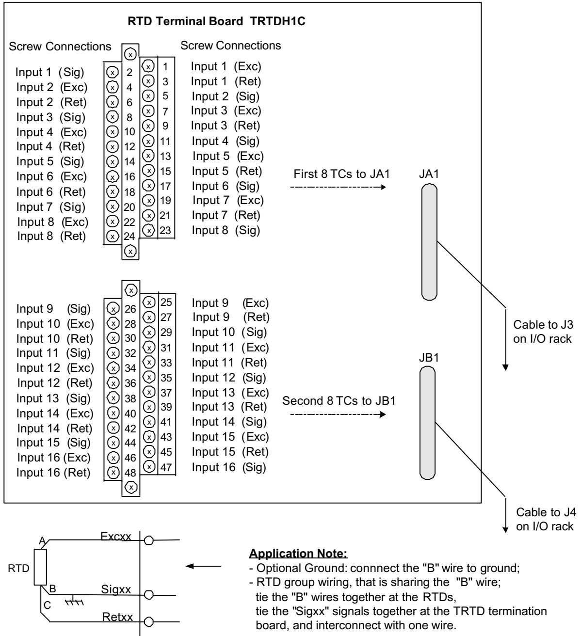
TRTDH1C (Simplex) Board Wiring
